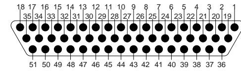
MicroD 51 Position Sockets
